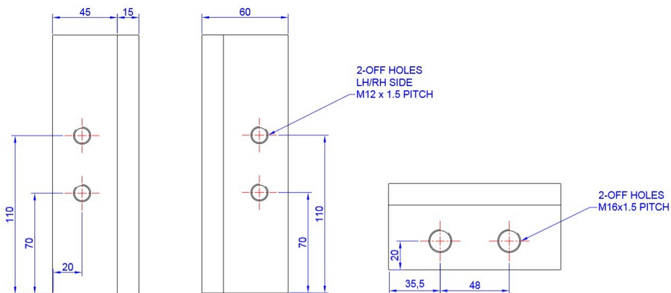
Fig. 6. Mounting specification for Signaline LocatorPlus-EN
